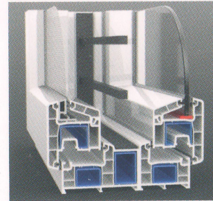
Casement Window with Grill & Mesh
