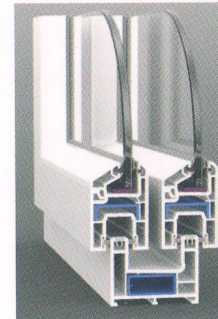
2-Track 2-Panel Window
